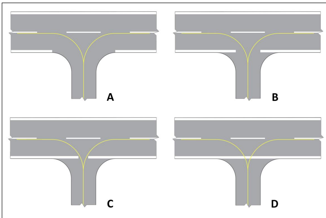
Figure GM-L-2. Illustration of runway side stripe marking interruption
