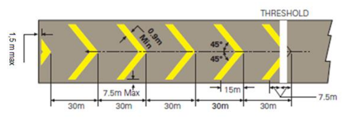
Figure R-2. Pre-threshold area marking
