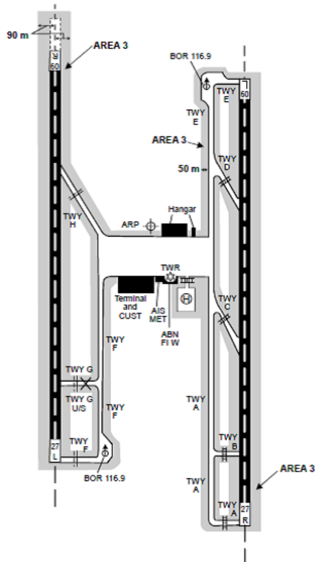
Figure 3 - Terrain and obstacle data collection surface — Area 3
