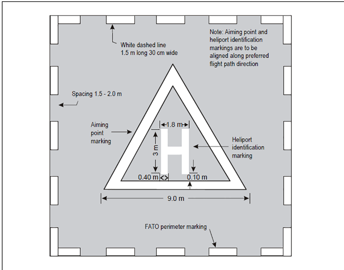
Figure F-1. Combined heliport identification, aiming point and FATO perimeter marking
