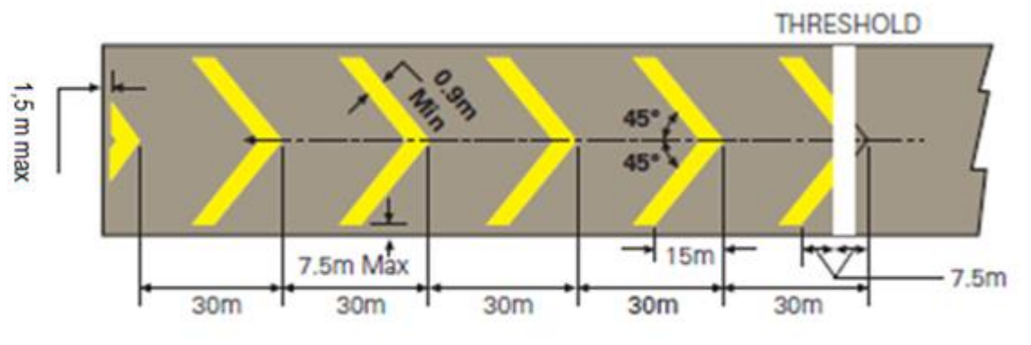
Figure R-2. Pre-threshold area marking
