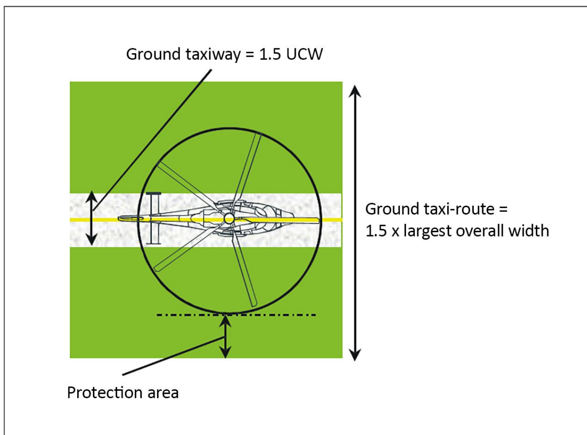
Figure C-1. Helicopter ground taxi-route/taxiway
